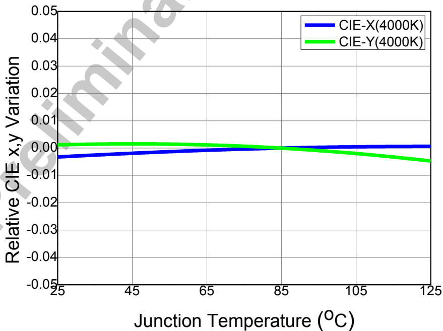
Fig 11. Junction Temperature vs. CIE x,y Shift, I_f=0.43A (4000K)
