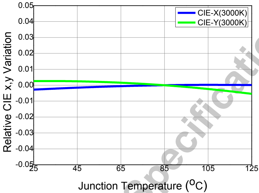
Fig 12. Junction Temperature vs. CIE x,y Shift, I_f=0.43A (3000K)
